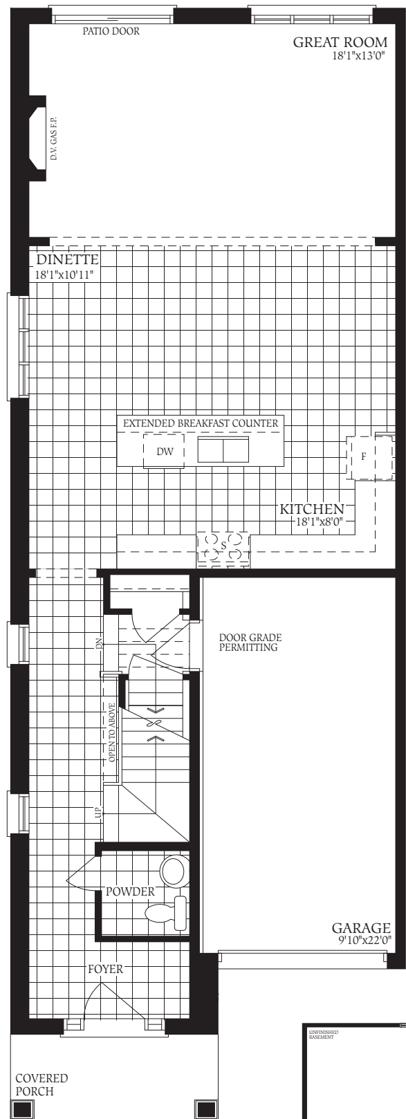
Ground Floor Elevation A & A1
